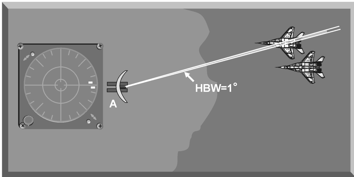
Figure 5-14. Azimuth Resolution
