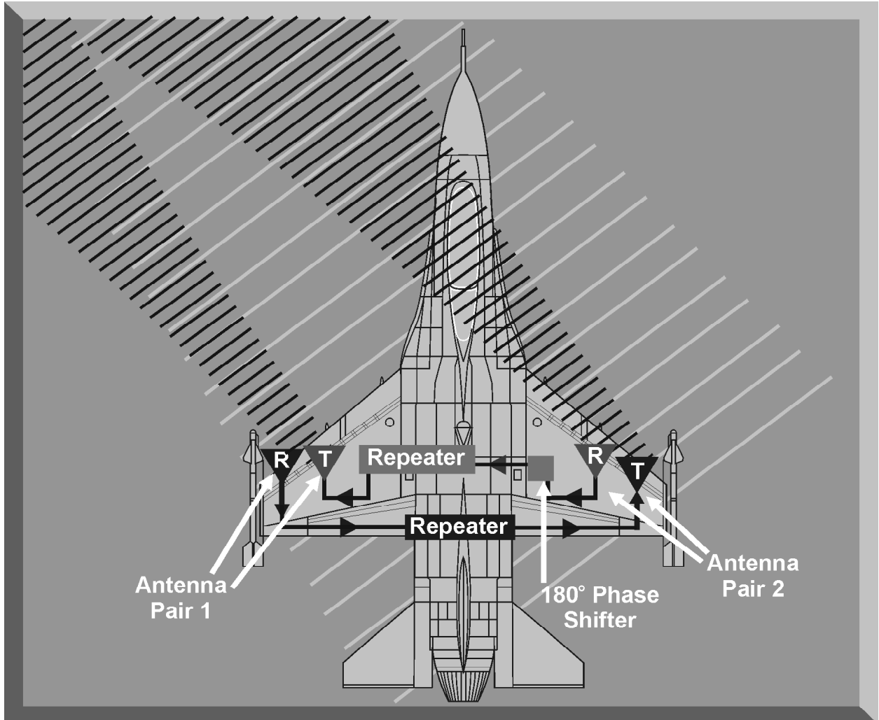
Figure 11-23. Cross-Eye Jamming
