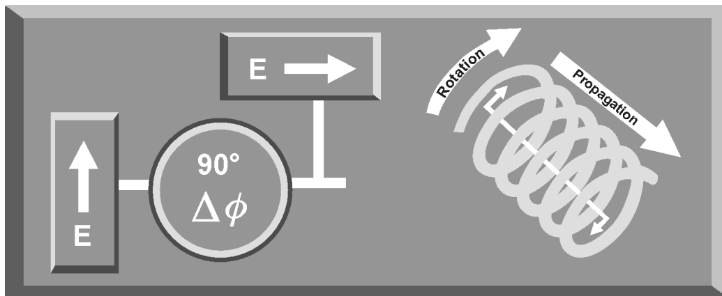
Figure 2-4. Circular Polarization
