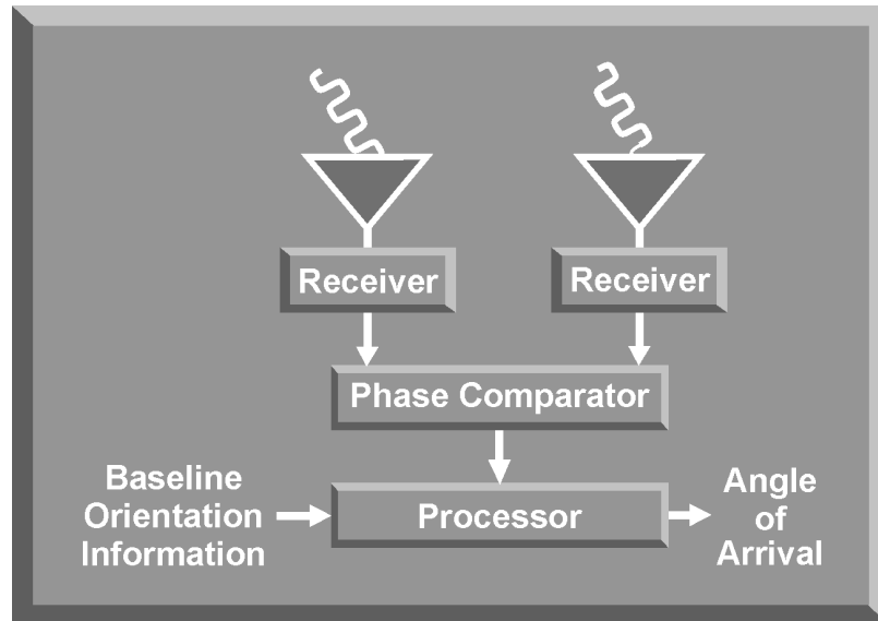
Figure 17-16. Interferometer Components
