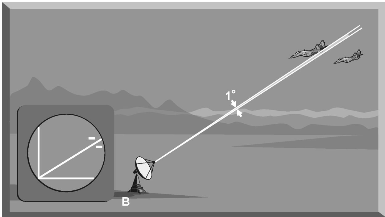
Figure 5-16. Elevation Resolution
