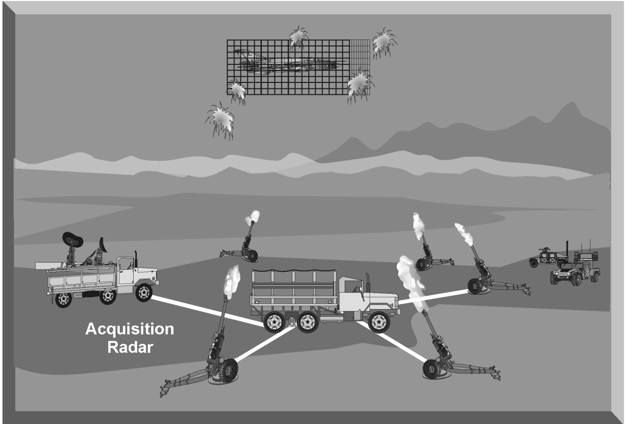
Figure 8-15. Sector/Barrage AAA
