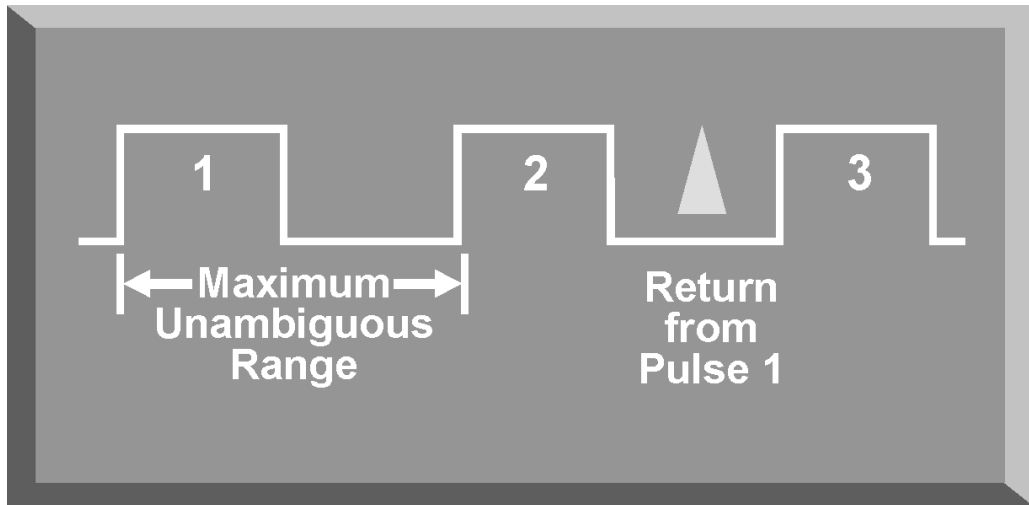
Figure 7-25. Range Ambiguity
