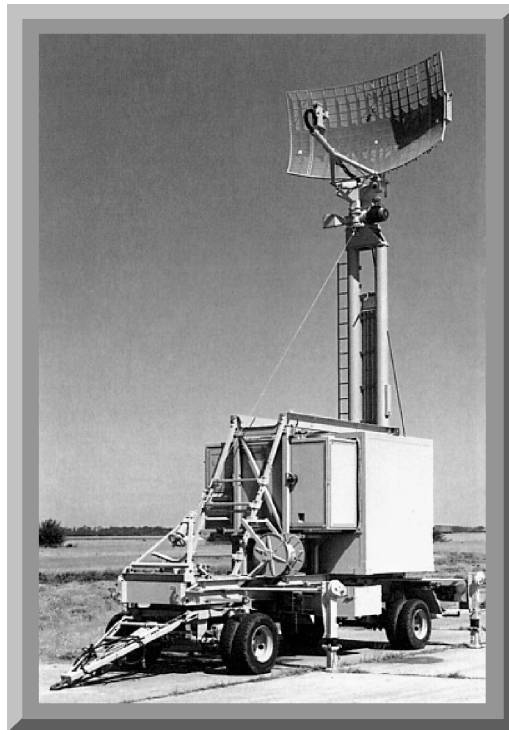
Figure 6-1. Parabolic Antenna
