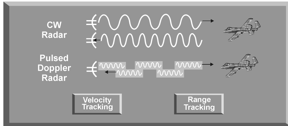
Figure 1-7. Velocity Discrimination
