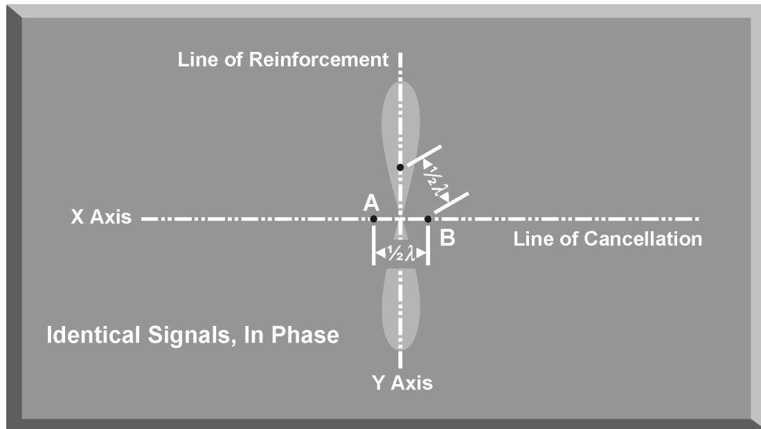
Figure 6-9. Broadside Array
