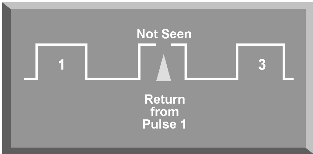
Figure 7-26. Range Eclipsing
