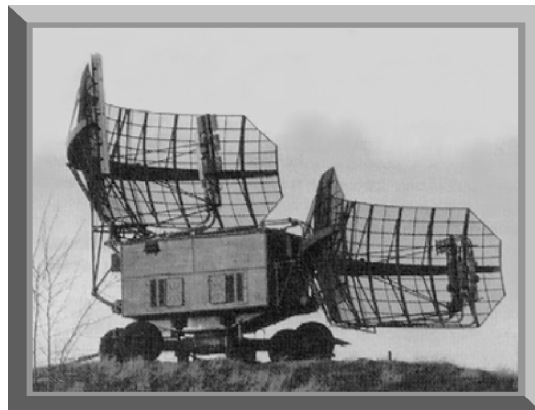
Figure 6-19. Stacked Beam Radar
