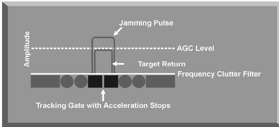
Figure 10-12. Velocity Gate Pull-Off Cover Pulse
