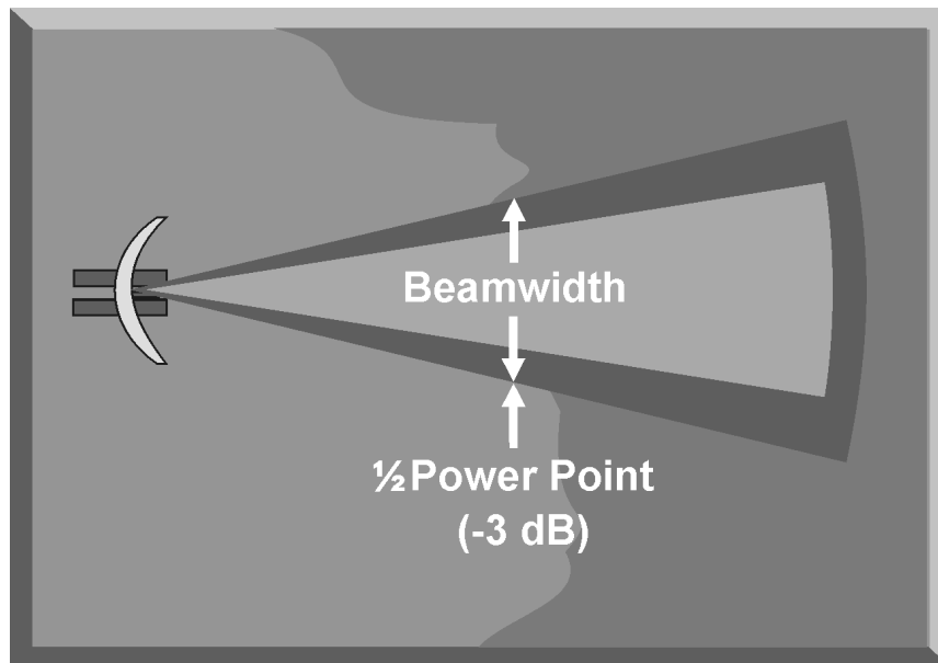
Figure 5-9. Radar Beamwidth
