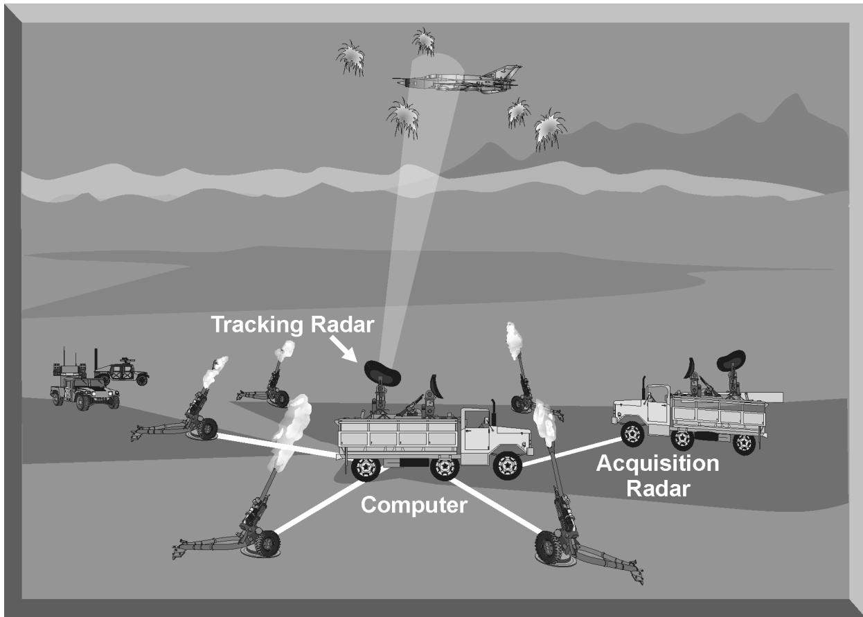
Figure 8-14. Radar-Directed AAA
