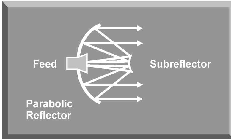
Figure 6-5. Cassegrain Antenna
