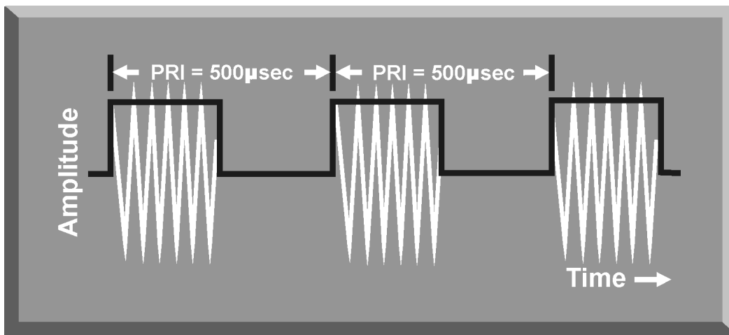
Figure 3-2. Constant PRF Radar Pulse
