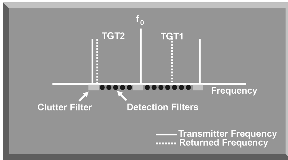
Figure 7-23. Range Ambiguity
