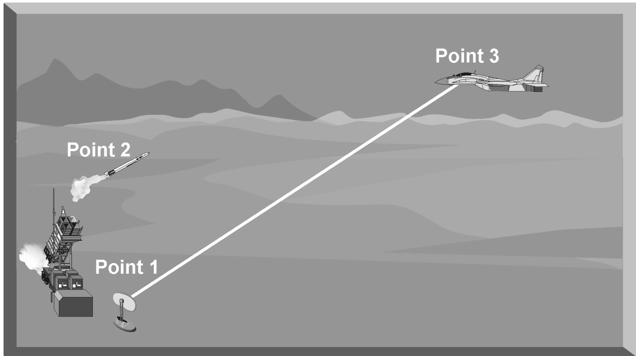
Figure 8-5. Command Guidance: Three-Point Pursuit
